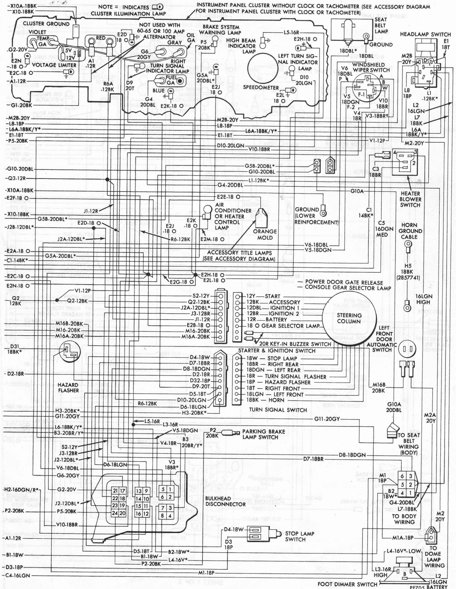
Fig. 10-Instrument Panel Wiring-Coronet, Charger (Rallye Cluster)
